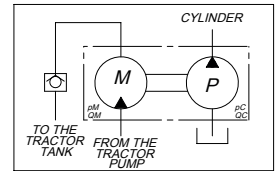
HYDRAULIC SYMBOL
