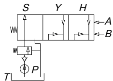
HYDRAULIC SYMBOL
